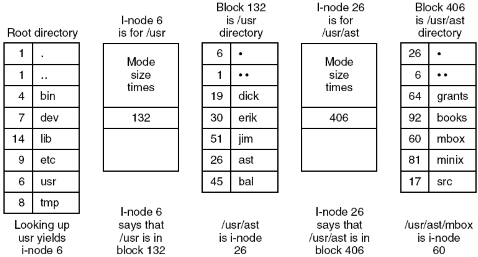
Figure 4-35. The steps in looking up /usr/ast/mbox .
